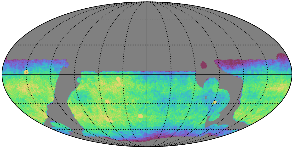
telescope_jerk_v3.5_10yrs WFD i band: CoaddM5
