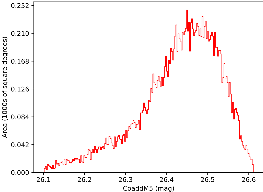
telescope_jerk_v3.5_10yrs WFD i band: CoaddM5
