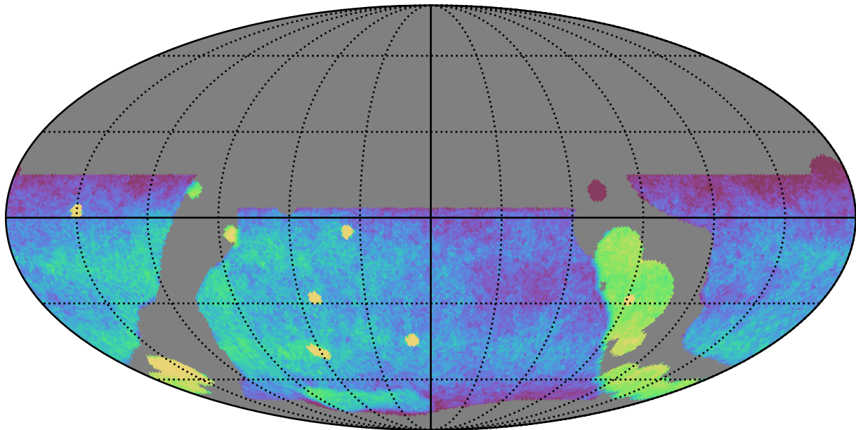
telescope_jerk_v3.5_10yrs WFD g band: CoaddM5
