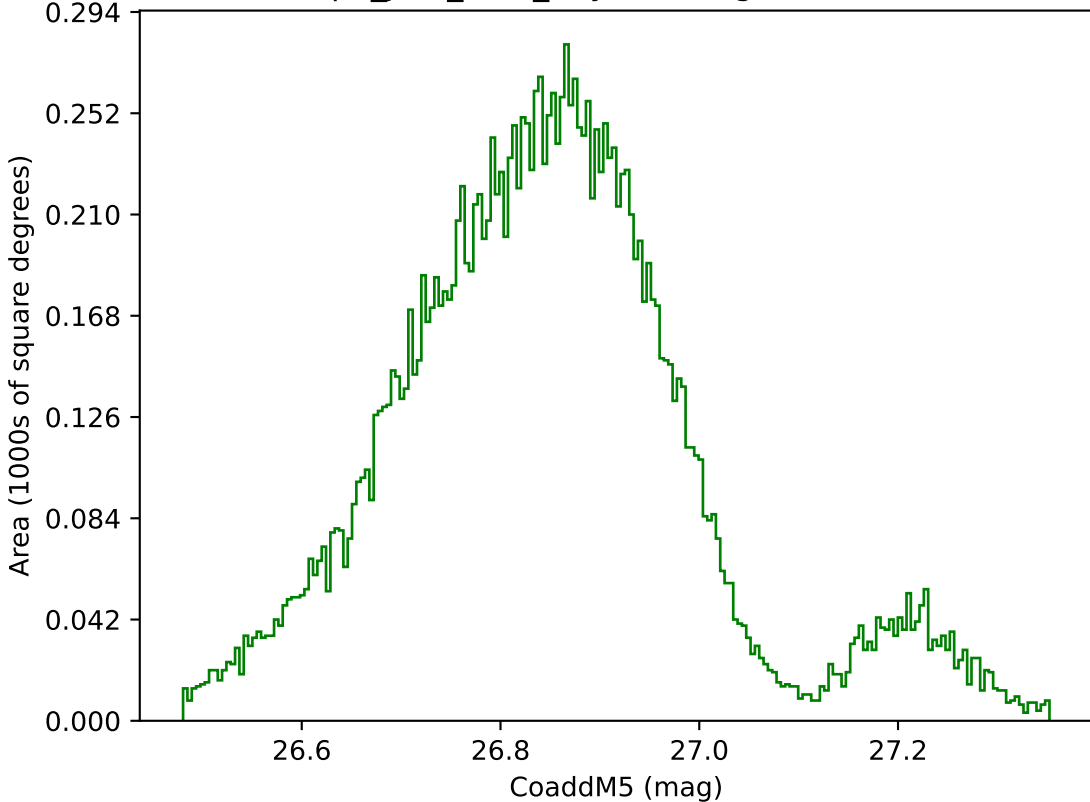
telescope_jerk_v3.5_10yrs WFD g band: CoaddM5
