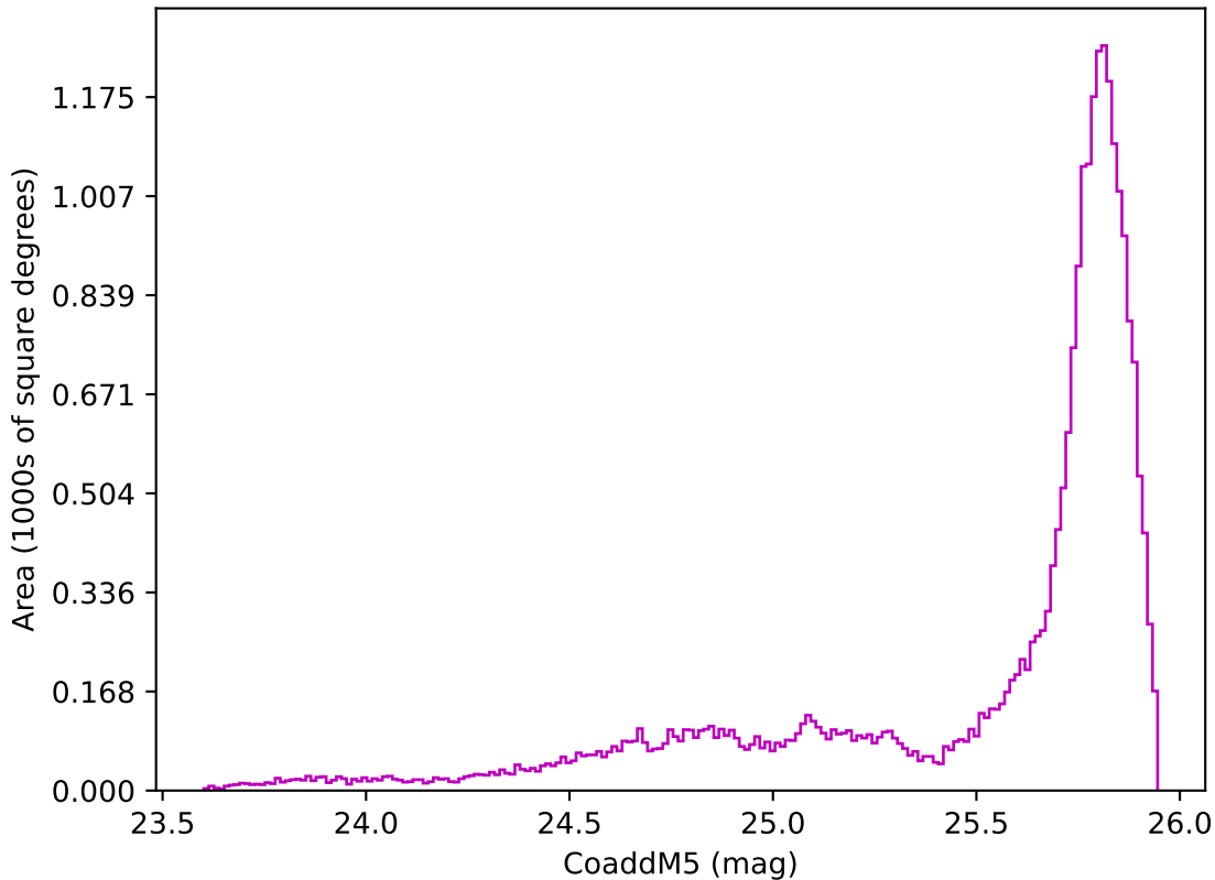
telescope_jerk_v3.5_10yrs All sky z band: CoaddM5
