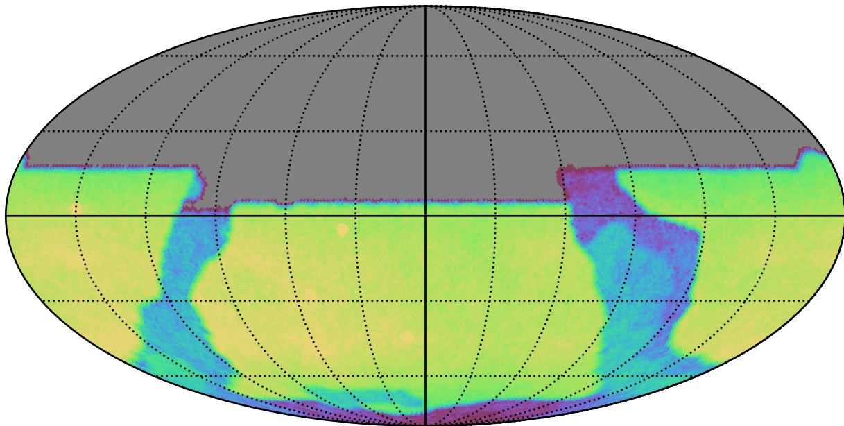
telescope_jerk_v3.5_10yrs All sky y band: CoaddM5
