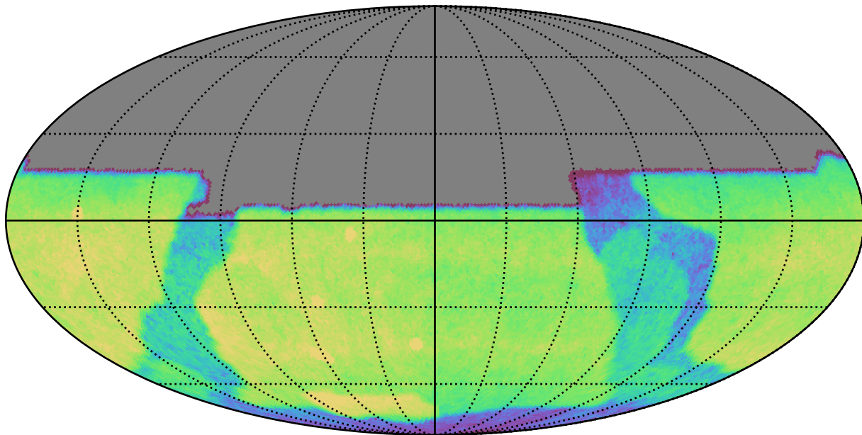
telescope_jerk_v3.5_10yrs All sky u band: CoaddM5
