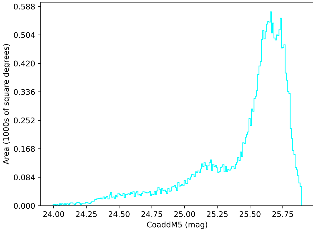
telescope_jerk_v3.5_10yrs All sky u band: CoaddM5
