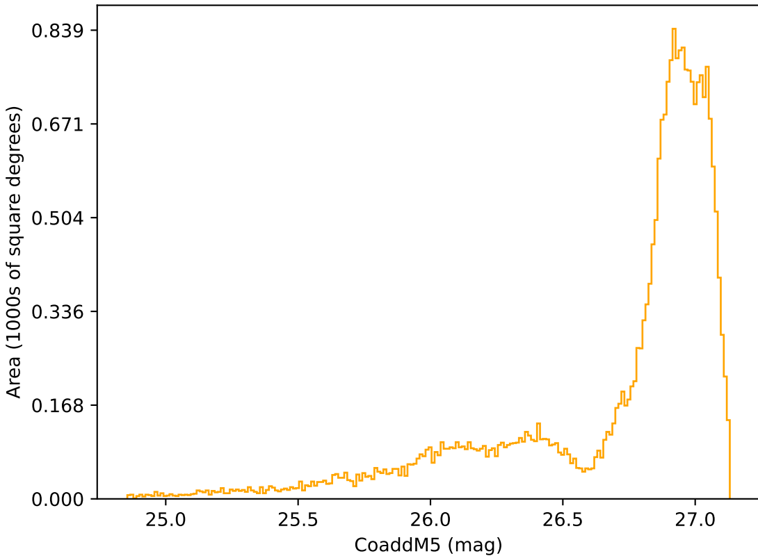
telescope_jerk_v3.5_10yrs All sky r band: CoaddM5
