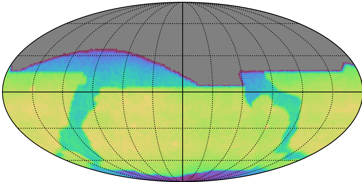
telescope_jerk_v3.5_10yrs All sky i band: CoaddM5
