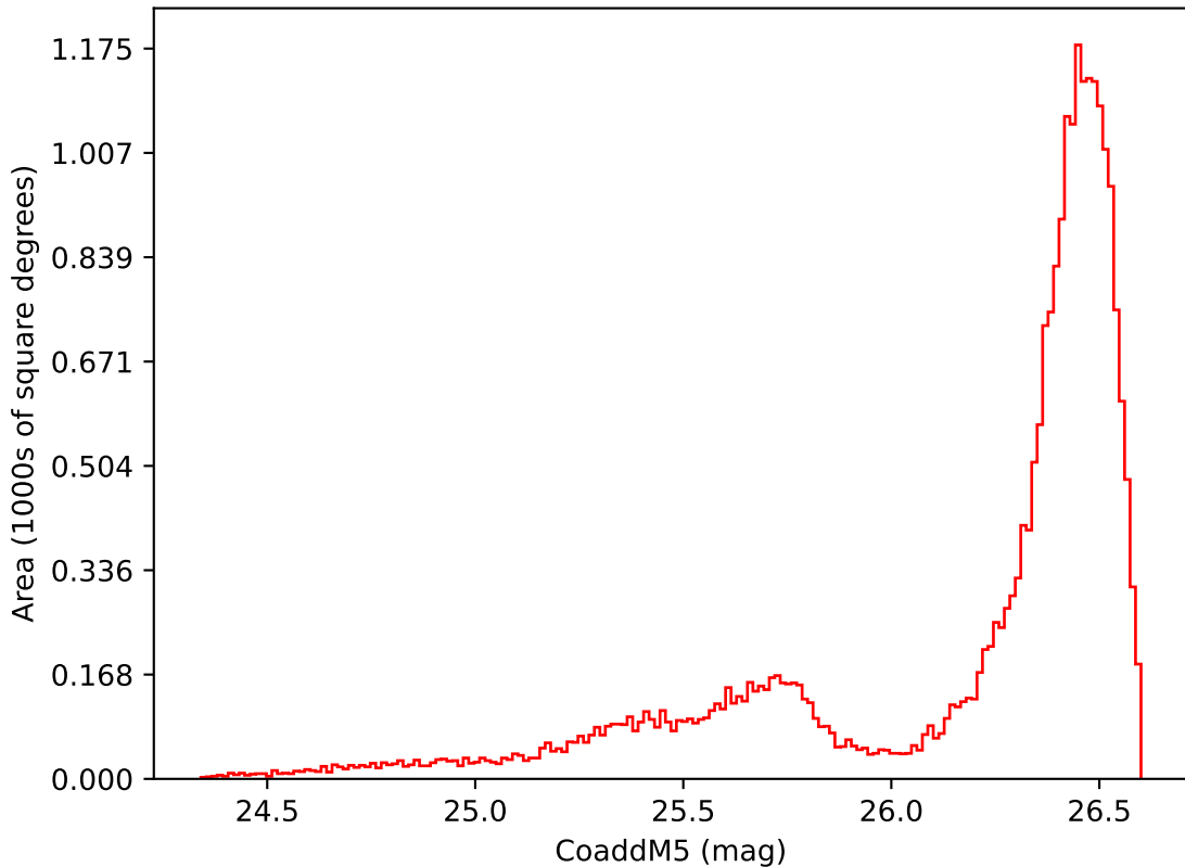
telescope_jerk_v3.5_10yrs All sky i band: CoaddM5
