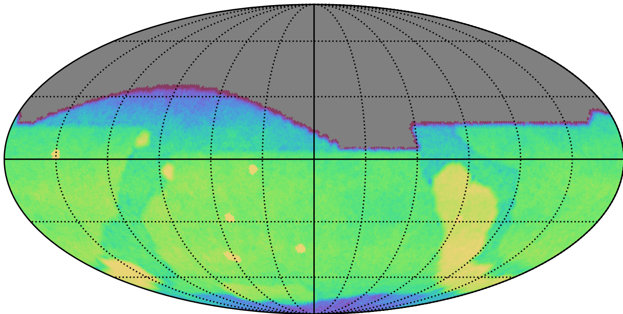
telescope_jerk_v3.5_10yrs All sky g band: CoaddM5
