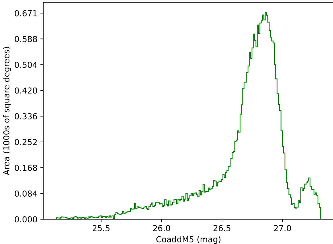
telescope_jerk_v3.5_10yrs All sky g band: CoaddM5
