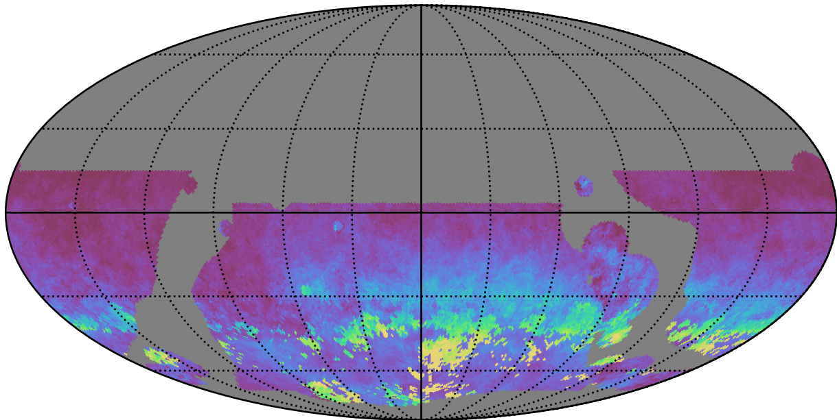
telescope_jerk_v3.5_10yrs WFD y band: AngleRms rotSkyPos
