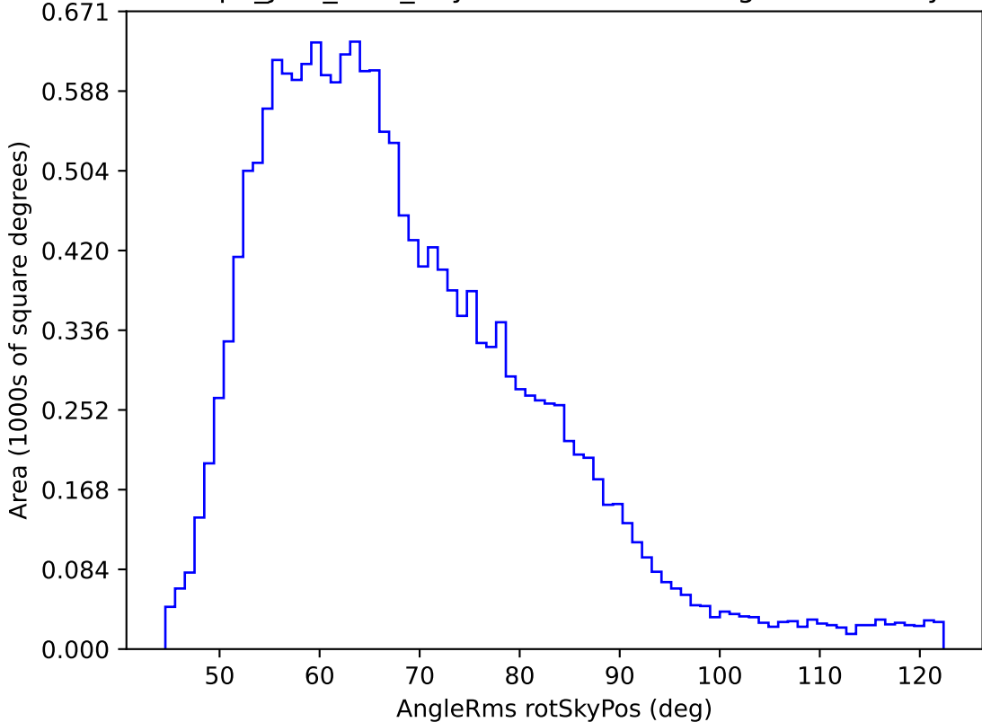
telescope_jerk_v3.5_10yrs WFD u band: AngleRms rotSkyPos
