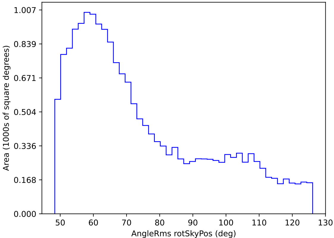
telescope_jerk_v3.5_10yrs WFD r band: AngleRms rotSkyPos
