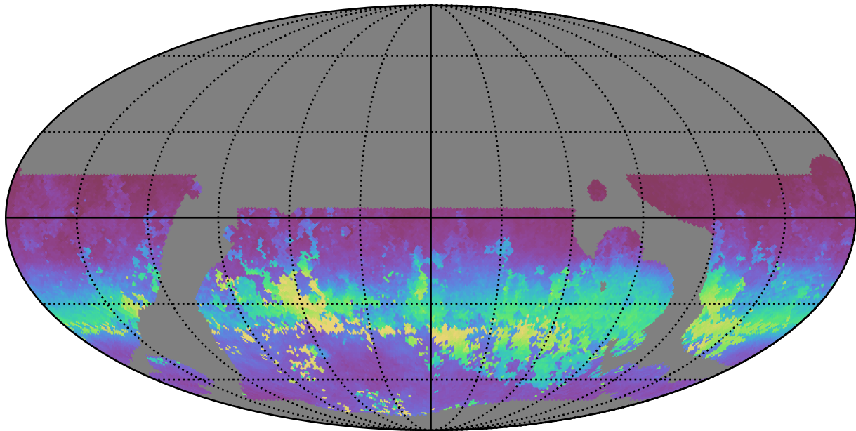
telescope_jerk_v3.5_10yrs WFD all bands: AngleRms rotSkyPos
