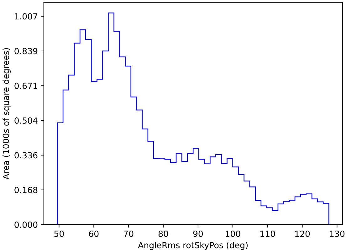
telescope_jerk_v3.5_10yrs WFD all bands: AngleRms rotSkyPos
