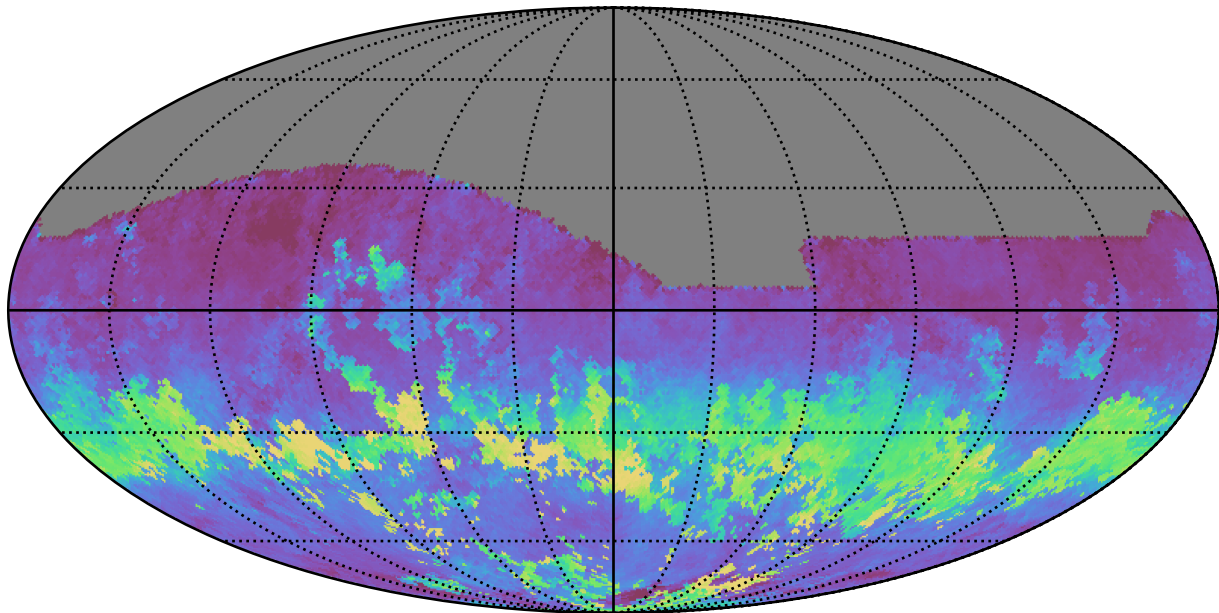
telescope_jerk_v3.5_10yrs All sky z band: AngleRms rotSkyPos
