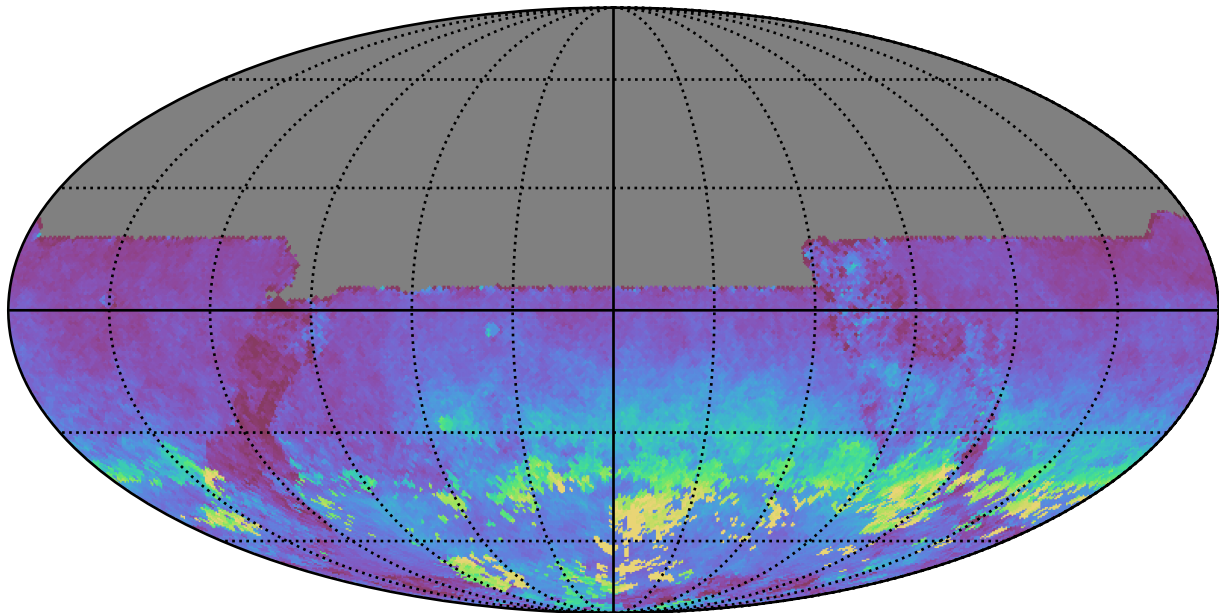
telescope_jerk_v3.5_10yrs All sky y band: AngleRms rotSkyPos
