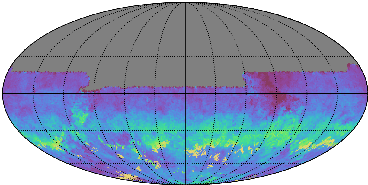
telescope_jerk_v3.5_10yrs All sky u band: AngleRms rotSkyPos
