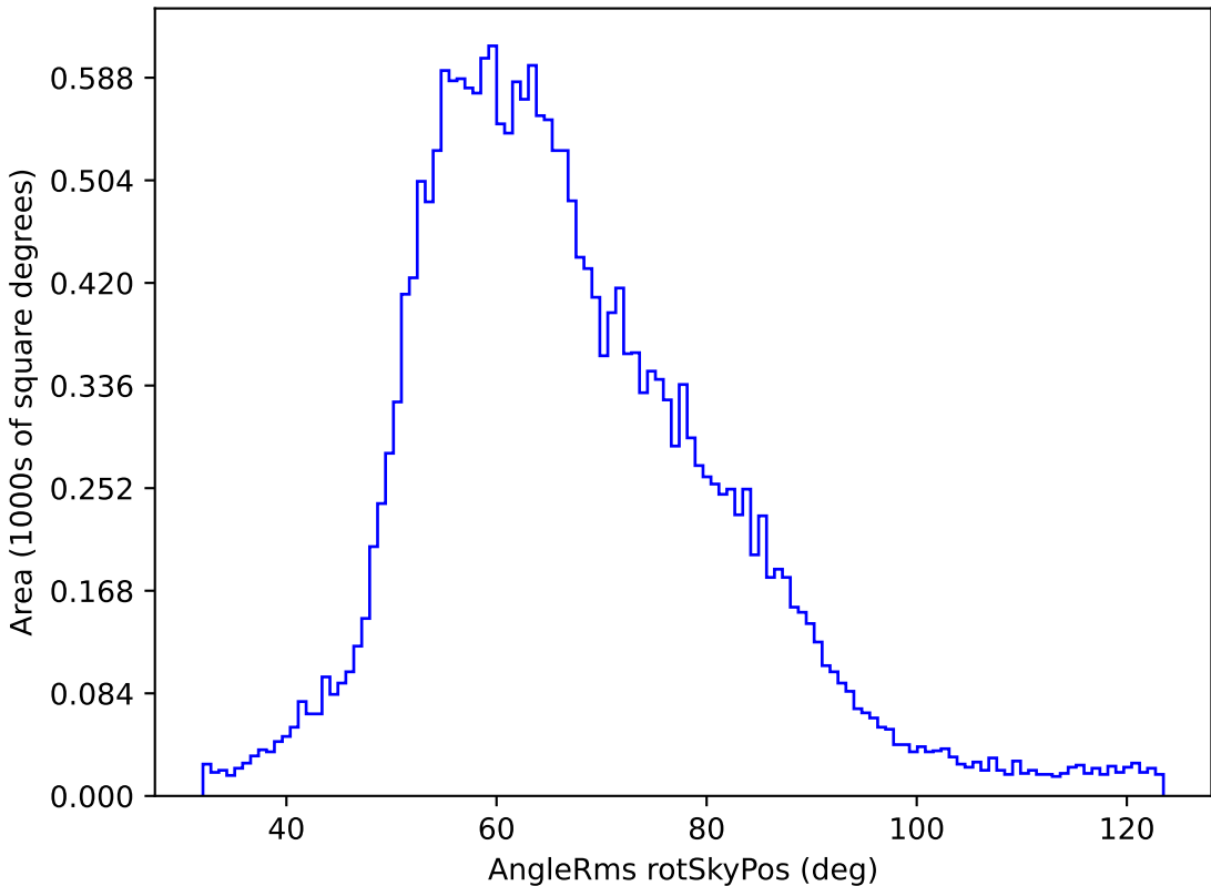
telescope_jerk_v3.5_10yrs All sky u band: AngleRms rotSkyPos
