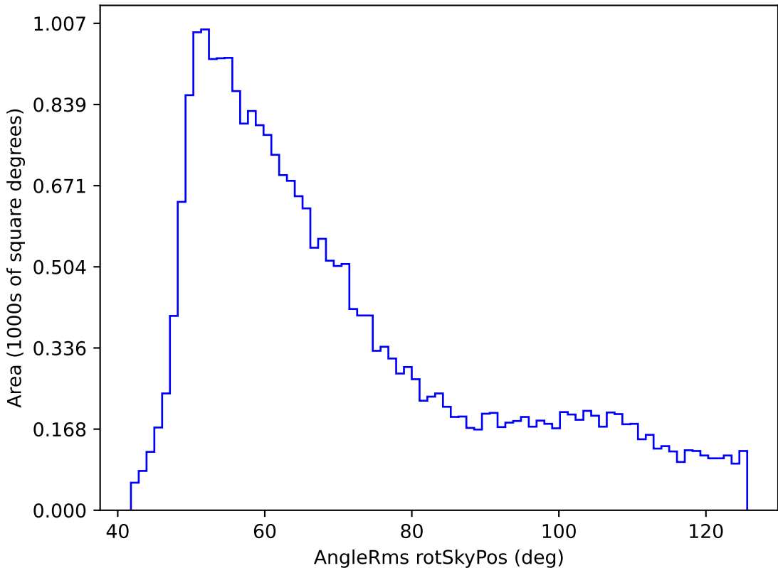
telescope_jerk_v3.5_10yrs All sky r band: AngleRms rotSkyPos
