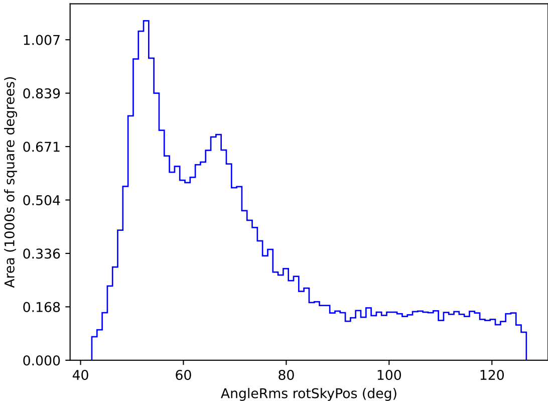
telescope_jerk_v3.5_10yrs All sky i band: AngleRms rotSkyPos
