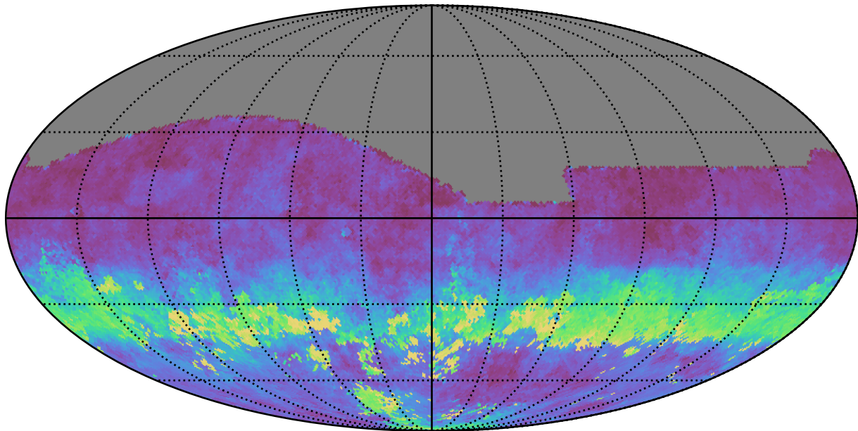
telescope_jerk_v3.5_10yrs All sky g band: AngleRms rotSkyPos
