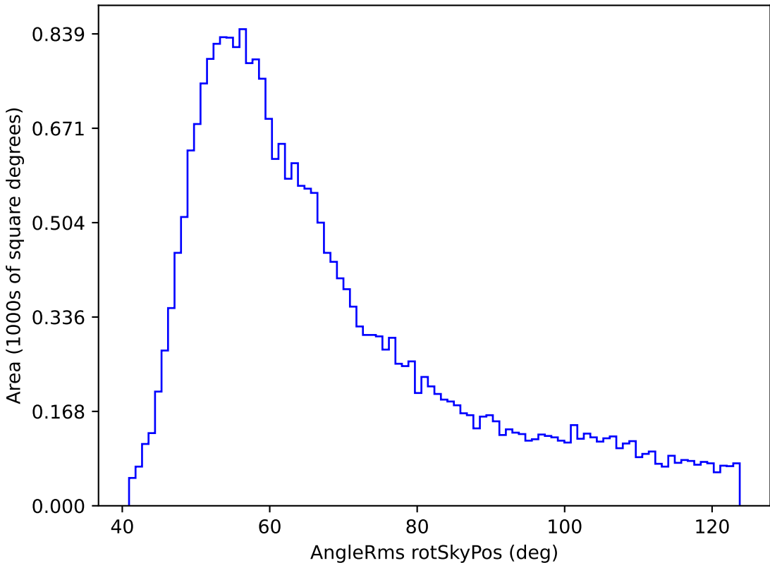
telescope_jerk_v3.5_10yrs All sky g band: AngleRms rotSkyPos
