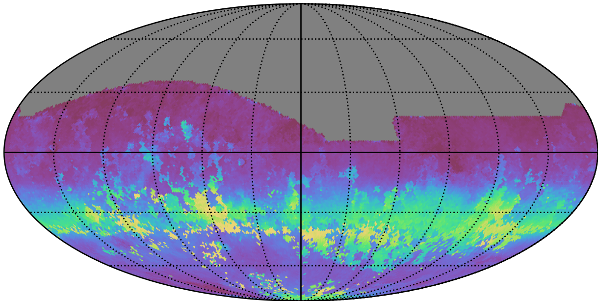
telescope_jerk_v3.5_10yrs All sky all bands: AngleRms rotSkyPos
