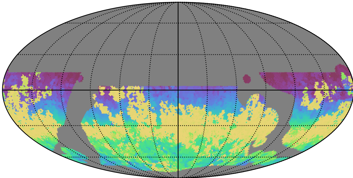
telescope_jerk_v3.5_10yrs WFD z band: AngleRange rotSkyPos
