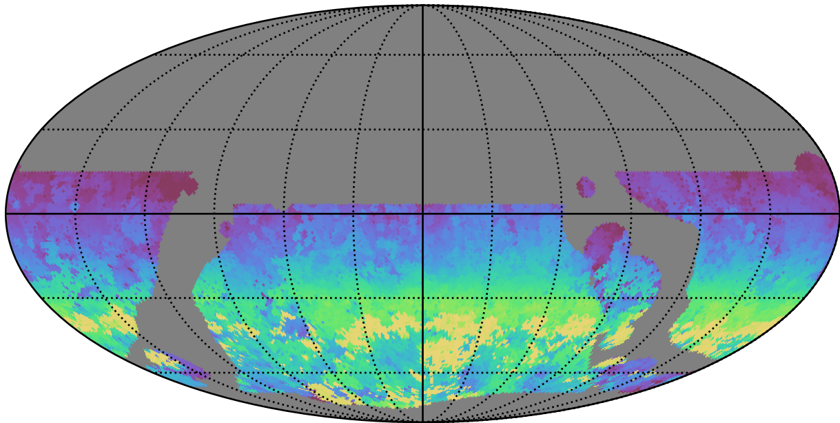
telescope_jerk_v3.5_10yrs WFD y band: AngleRange rotSkyPos
