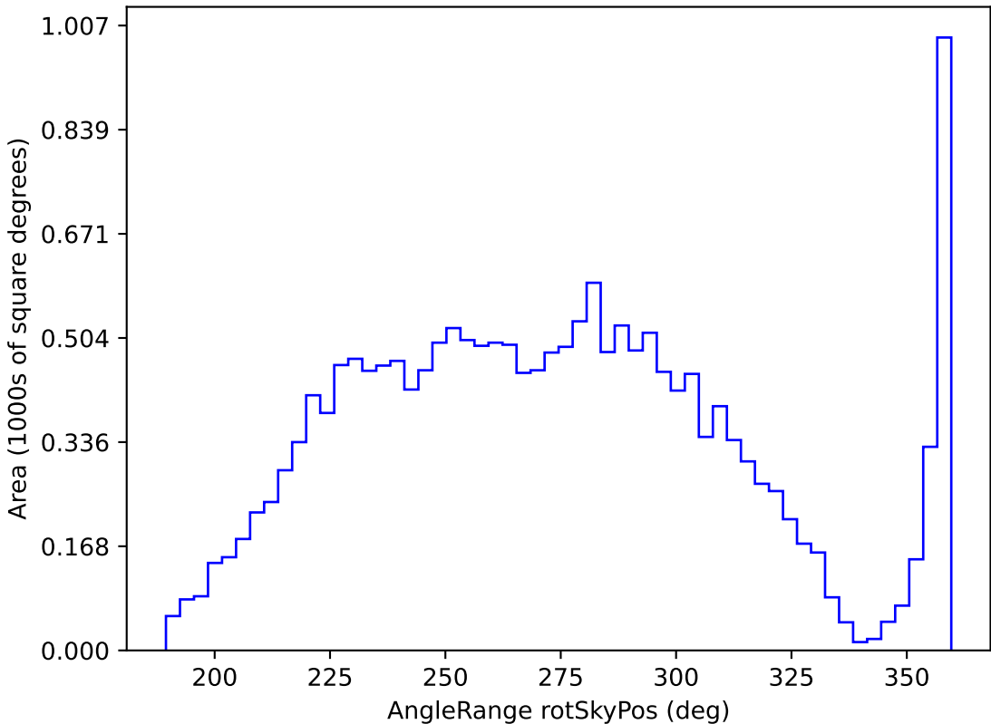
telescope_jerk_v3.5_10yrs WFD y band: AngleRange rotSkyPos
