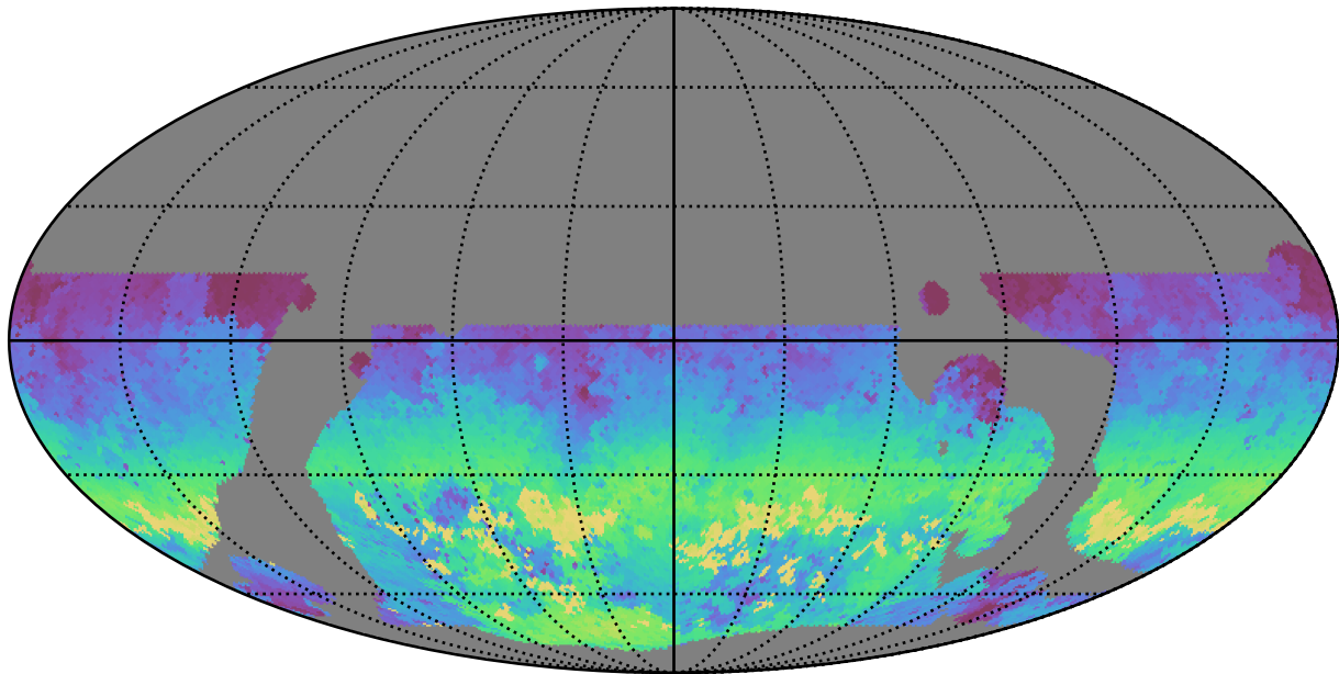
telescope_jerk_v3.5_10yrs WFD u band: AngleRange rotSkyPos
