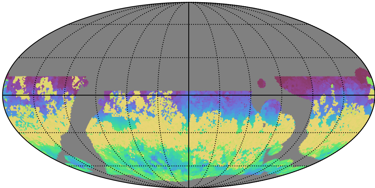
telescope_jerk_v3.5_10yrs WFD r band: AngleRange rotSkyPos
