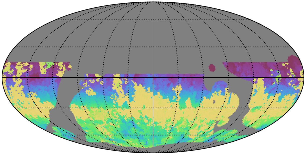
telescope_jerk_v3.5_10yrs WFD i band: AngleRange rotSkyPos
