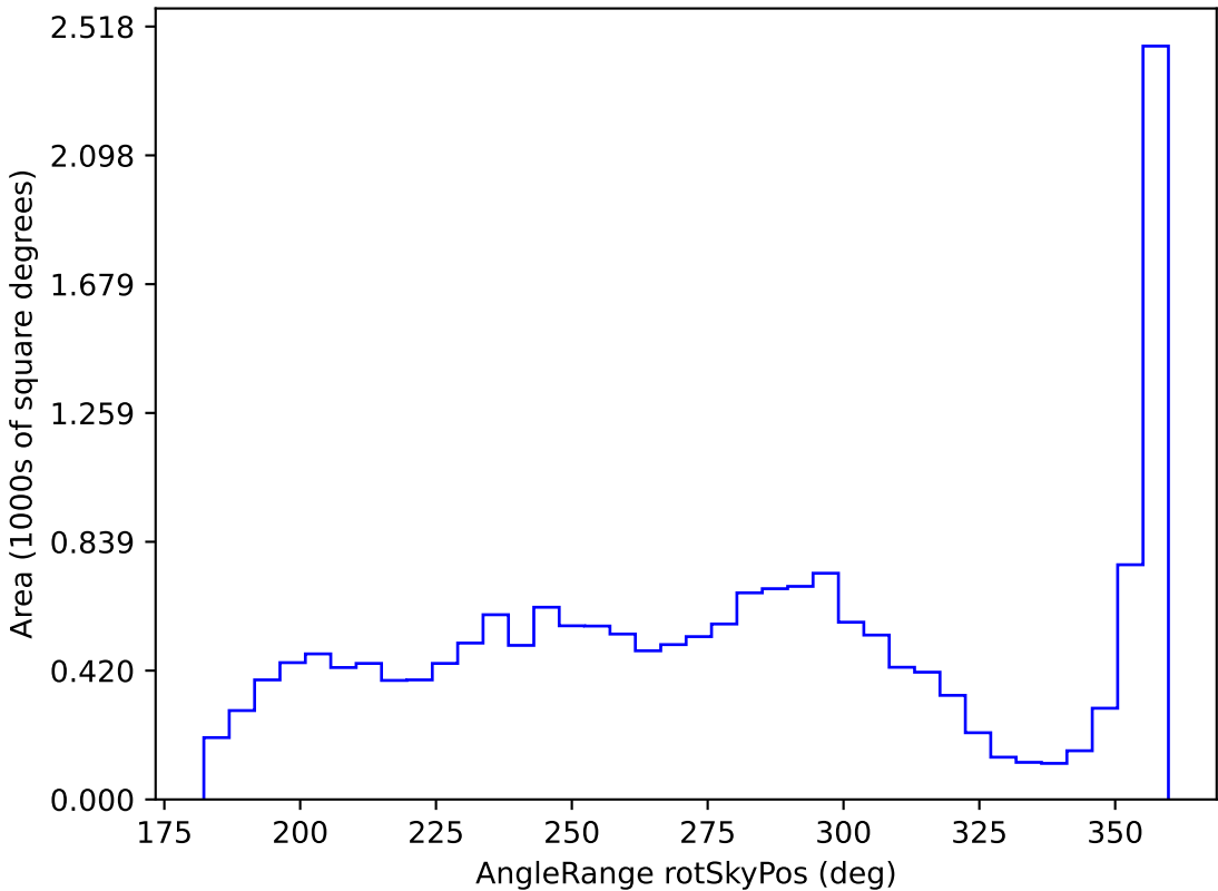
telescope_jerk_v3.5_10yrs WFD g band: AngleRange rotSkyPos
