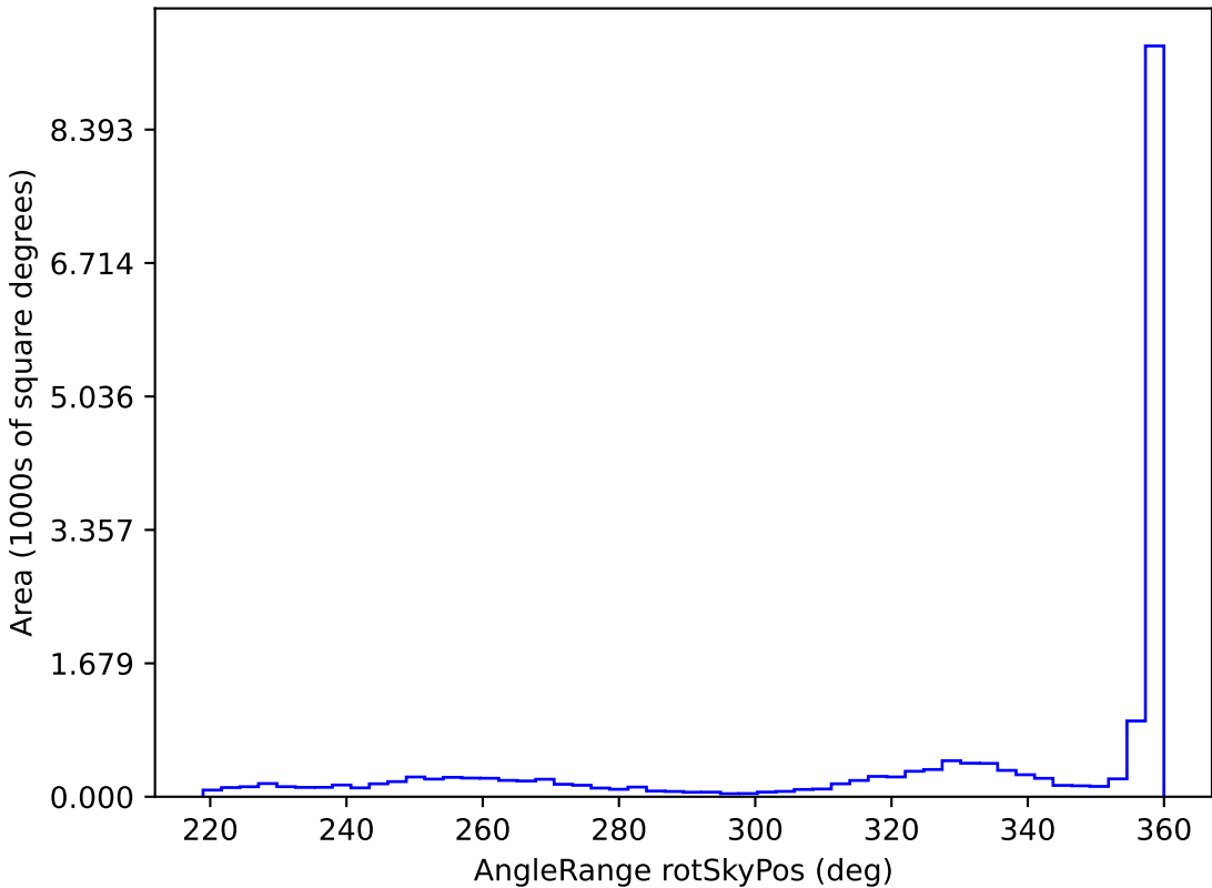
telescope_jerk_v3.5_10yrs WFD all bands: AngleRange rotSkyPos
