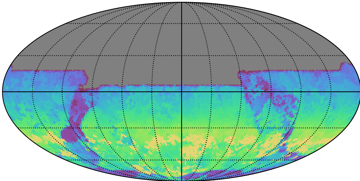
telescope_jerk_v3.5_10yrs All sky y band: AngleRange rotSkyPos
