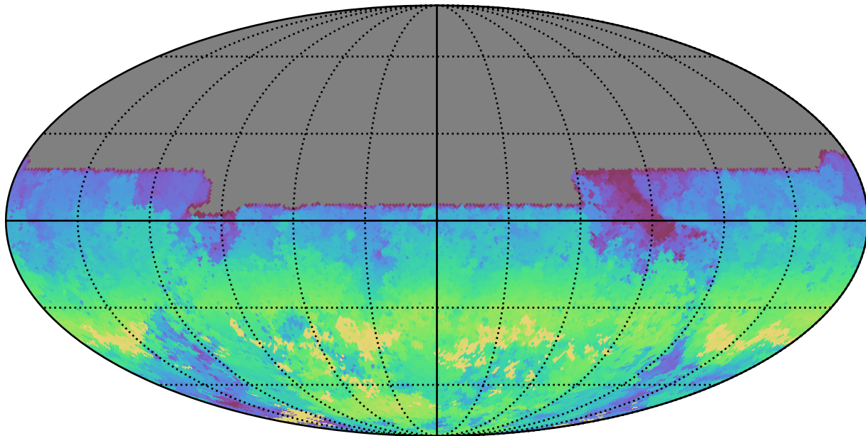
telescope_jerk_v3.5_10yrs All sky u band: AngleRange rotSkyPos
