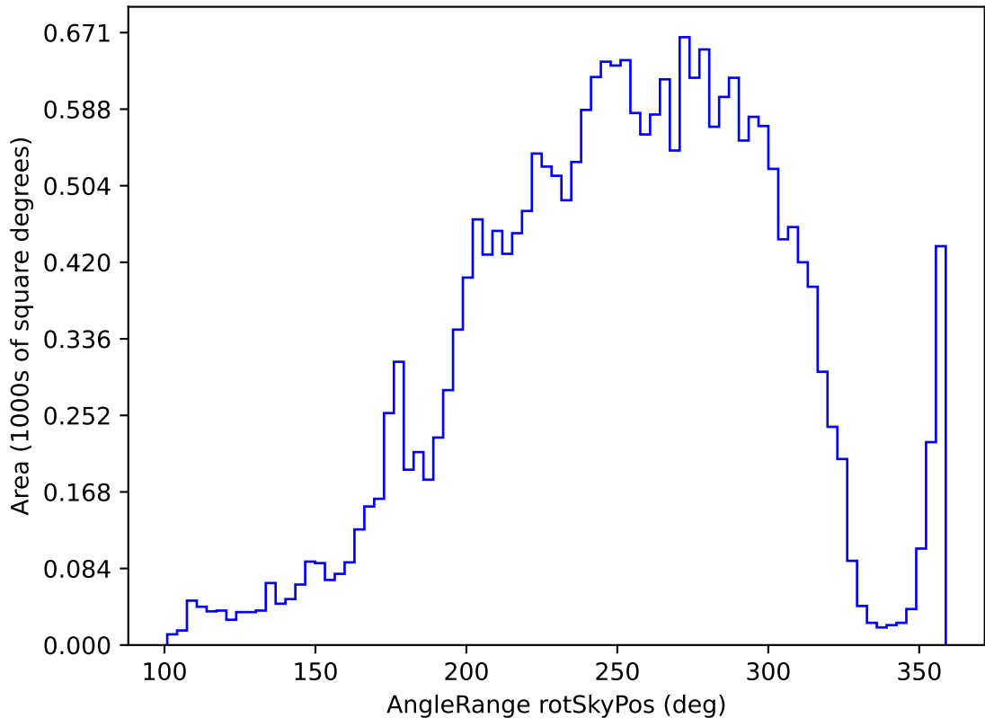
telescope_jerk_v3.5_10yrs All sky u band: AngleRange rotSkyPos
