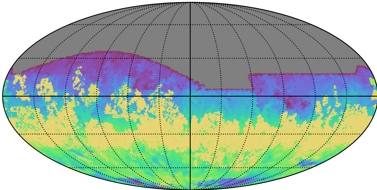
telescope_jerk_v3.5_10yrs All sky r band: AngleRange rotSkyPos
