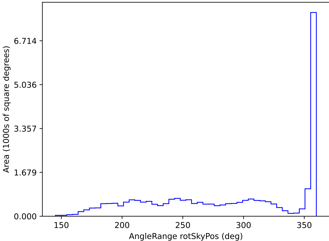
telescope_jerk_v3.5_10yrs All sky r band: AngleRange rotSkyPos
