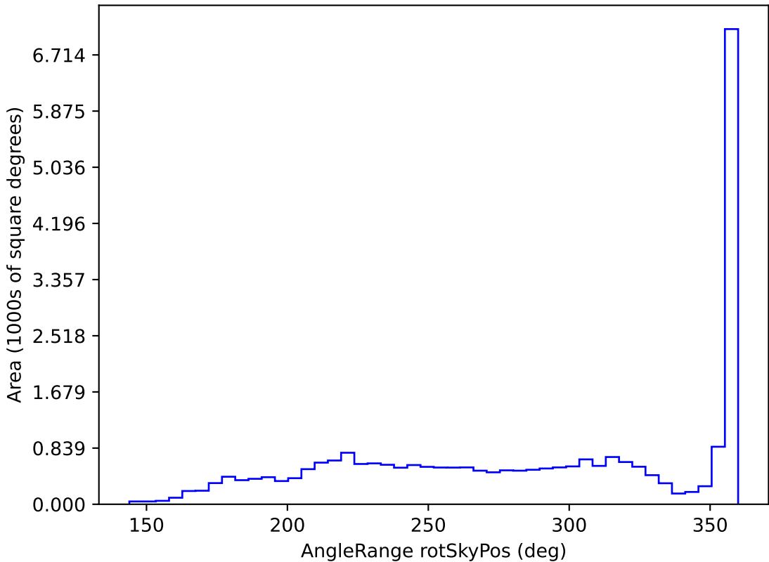
telescope_jerk_v3.5_10yrs All sky i band: AngleRange rotSkyPos
