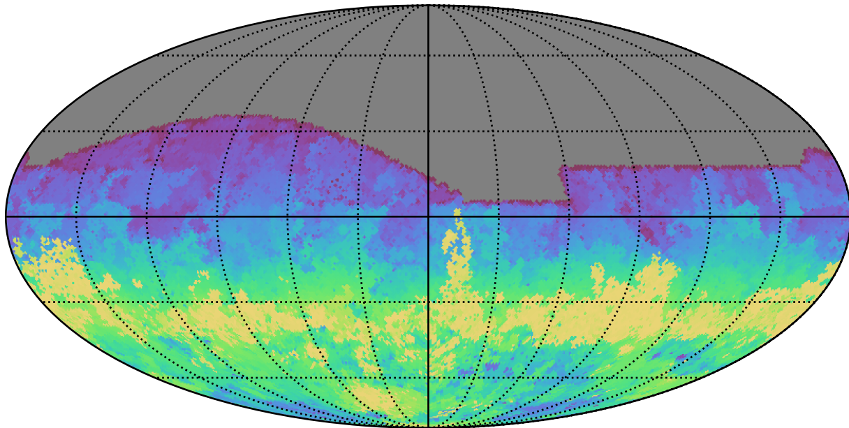
telescope_jerk_v3.5_10yrs All sky g band: AngleRange rotSkyPos
