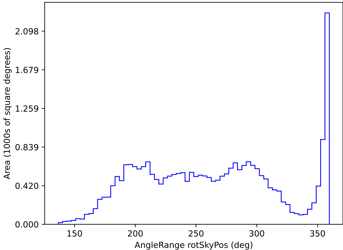
telescope_jerk_v3.5_10yrs All sky g band: AngleRange rotSkyPos
