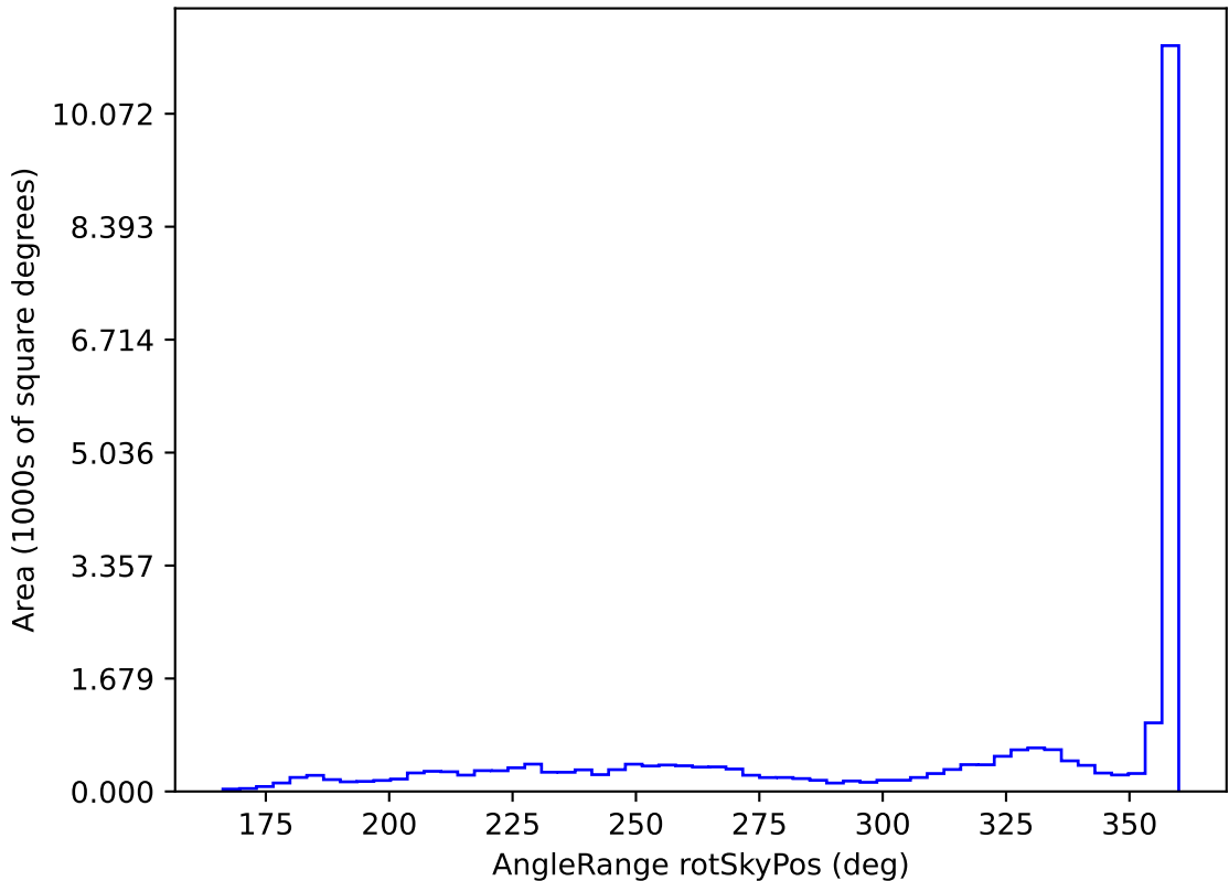
telescope_jerk_v3.5_10yrs All sky all bands: AngleRange rotSkyPos
