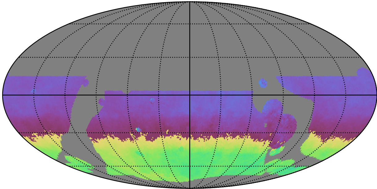
telescope_jerk_v3.5_10yrs WFD y band: AngleMean rotSkyPos
