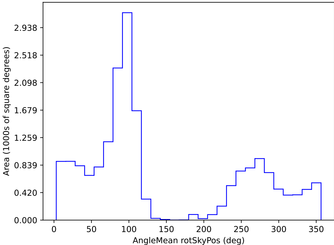
telescope_jerk_v3.5_10yrs WFD u band: AngleMean rotSkyPos
