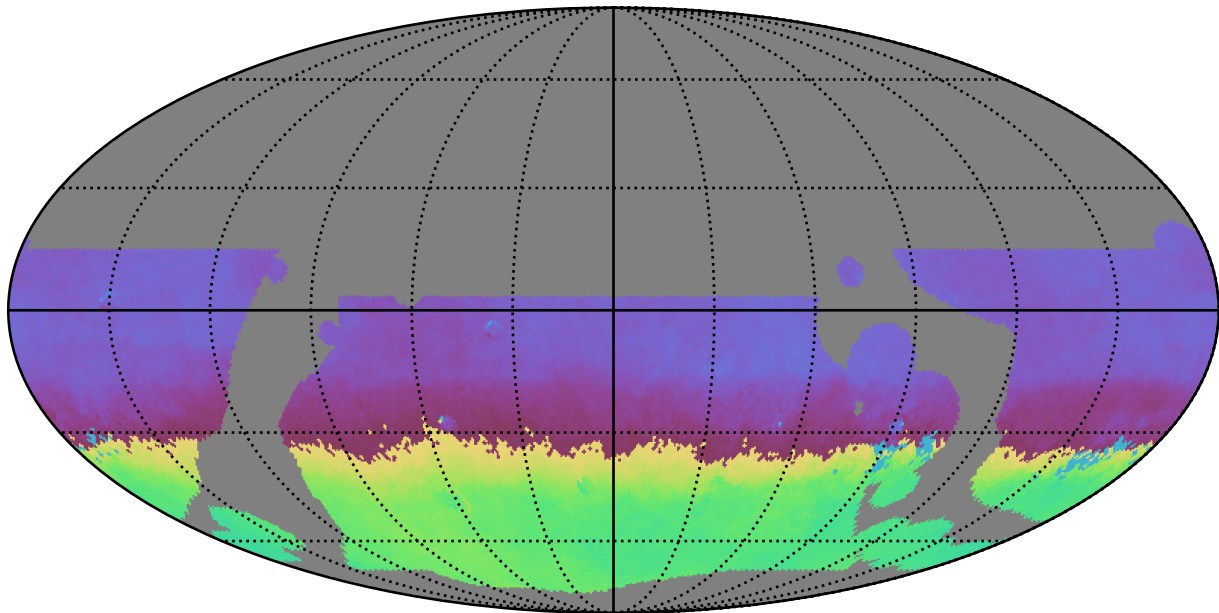
telescope_jerk_v3.5_10yrs WFD r band: AngleMean rotSkyPos
