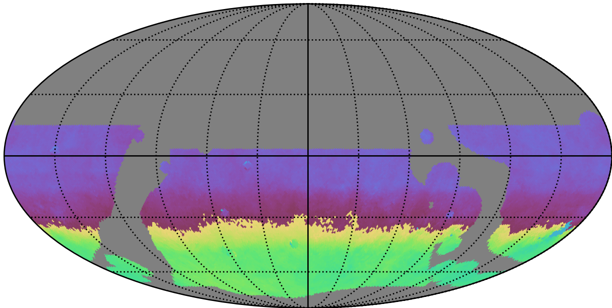
telescope_jerk_v3.5_10yrs WFD i band: AngleMean rotSkyPos
