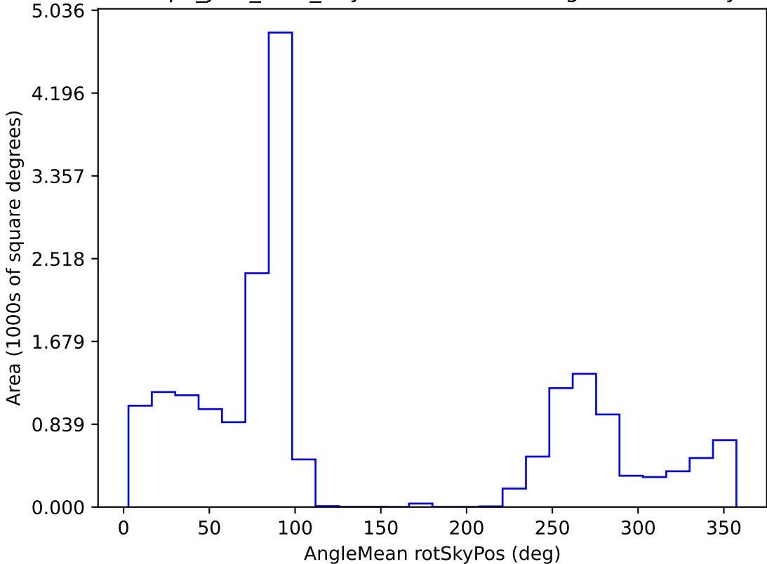
telescope_jerk_v3.5_10yrs WFD i band: AngleMean rotSkyPos
