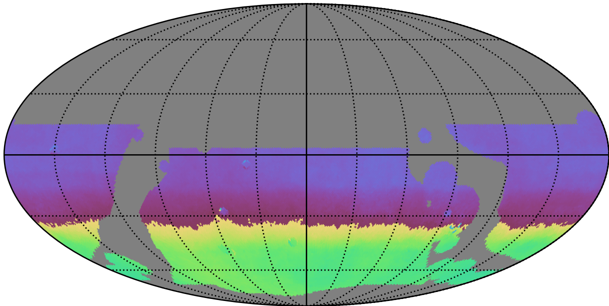
telescope_jerk_v3.5_10yrs WFD all bands: AngleMean rotSkyPos
